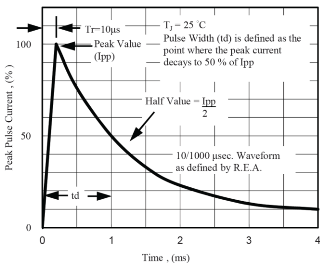
Fig. 5 - Pulse Waveform
